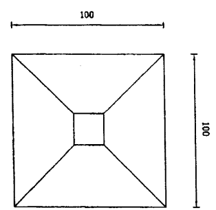
FOOTING F2
